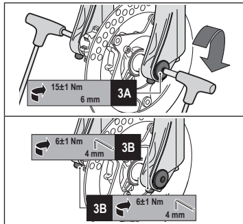
Picture 3 - \phi 20 mm through axle: wheel installation
