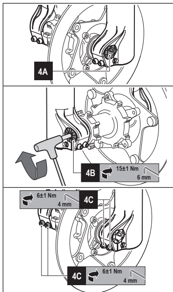
Picture 4 - \phi 20 mm Taperwall through axle: wheel installation
