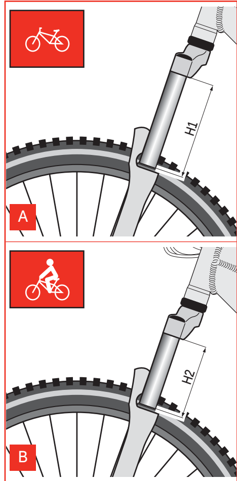
Picture 8 - How to measure the SAG
