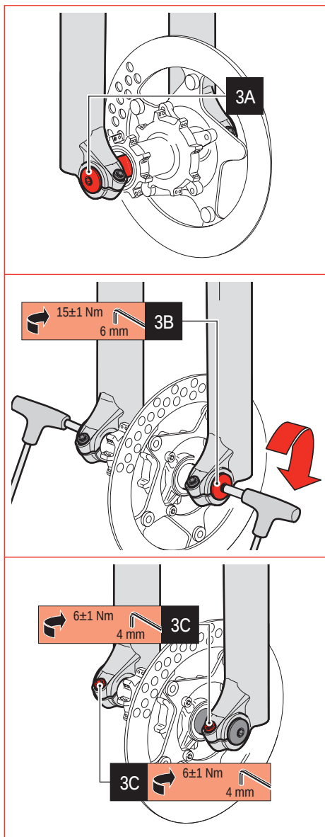
Picture 3 - Wheel installation on \varnothing 32 fork with a 20 mm diameter through-hole axle
