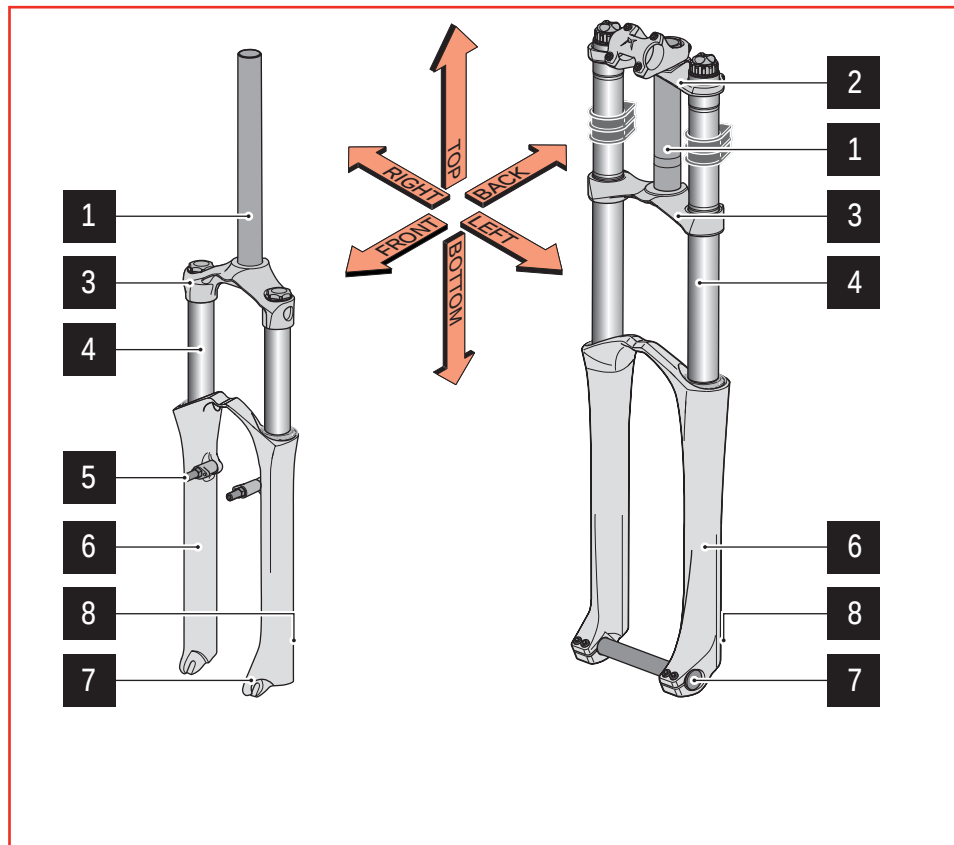
Picture 1 - Conventional orientation of the fork
