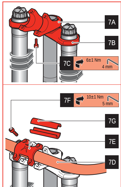
Picture 7 - Handlebar clamp installation
