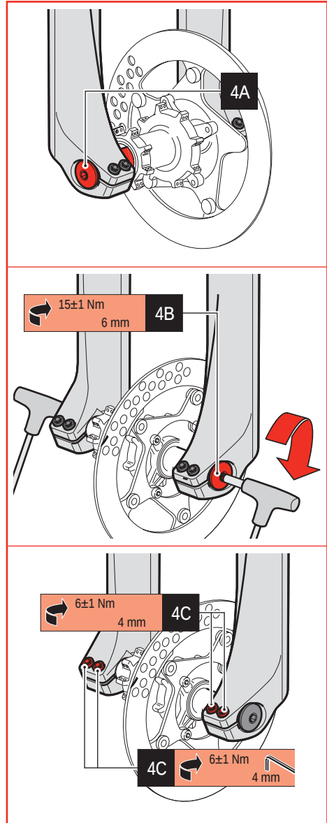
Picture 4 - Wheel installation on \varnothing 35 forks with a 20 mm diameter through-hole axle
