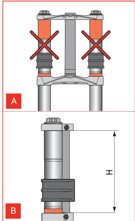
Picture 2 - Dual crown forks installation on the frame: (2A) Crowns fastening, (2B) Steer tube maximum length between crowns
