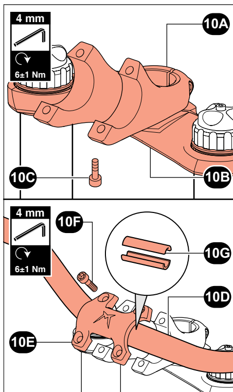
Picture 10 - Handlebar Clamp Installation For The 888 Series
