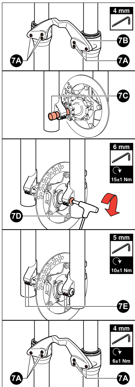
Picture 7 - Wheel Installation On Monster Series Forks
