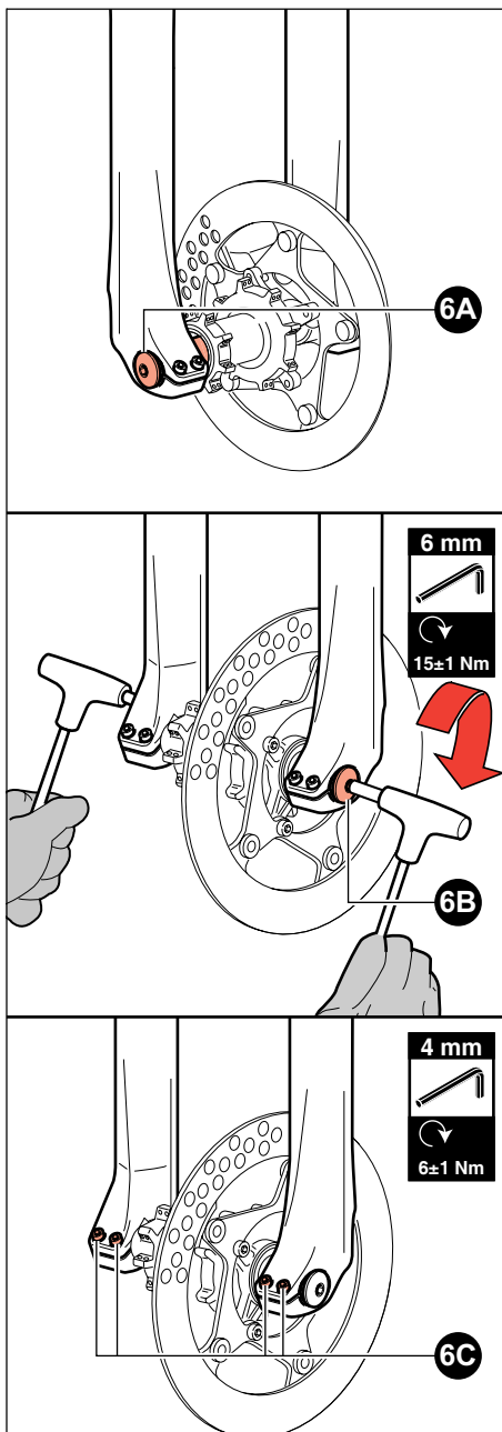
Picture 6 - Wheel Installation on 66 end 888 series forks
