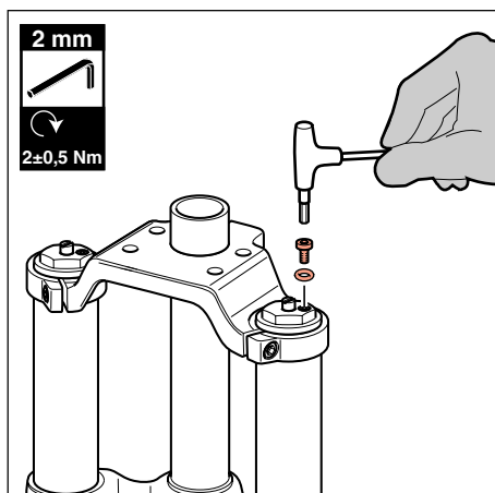
Picture 11 - Monster Air-Bleeding
