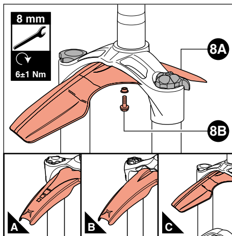
Picture 8 - Fender Installation
