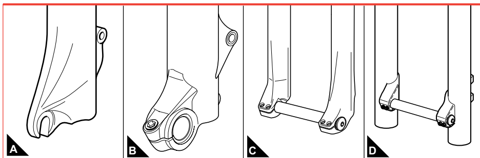
Picture 4 - Wheel securing systems: (4A) standard dropouts, (4B) \varnothing 20mm through-hole axle (forks with \varnothing 32mm stanchions), (4C) \varnothing 20mm through-hole axle (66 and 888 series forks), (4D) \varnothing 20mm through-hole axle (Monster).
