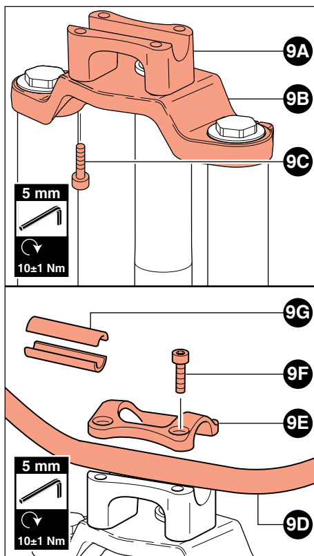
Picture 9 - Handlebar Clamp Installation
