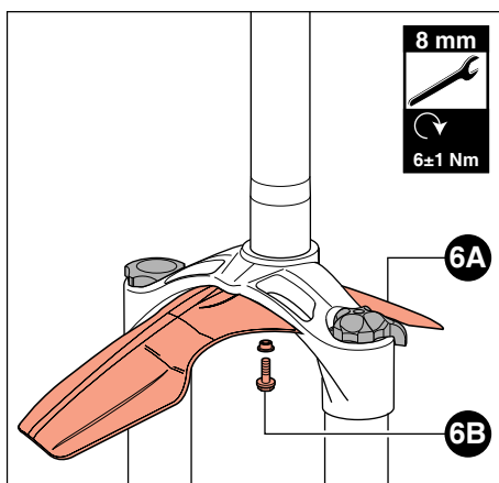
Picture 6 - Fender Installation
