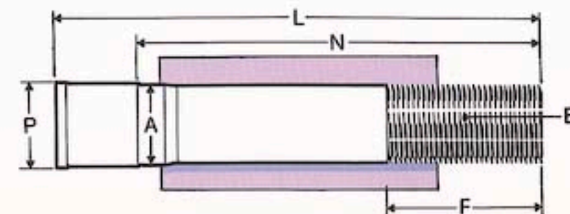
Cannotto per base standard/Stem for standard bottom yoke
